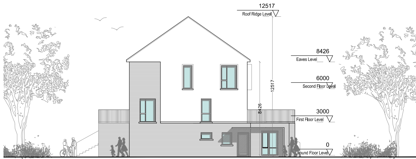
Northern Elevation SCALE 1:200 @ A3
